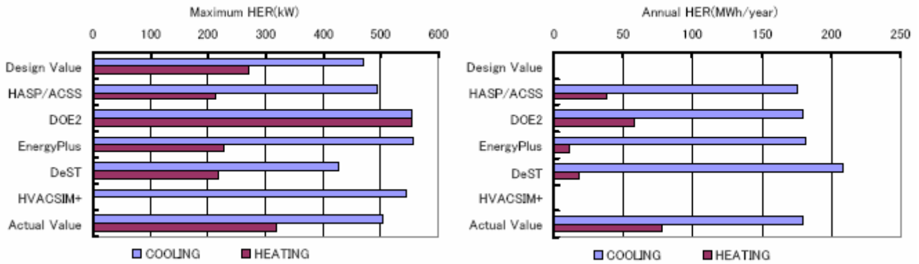
Figure 5 Comparison of coil heat extraction rate for various simulation programs and designed value
