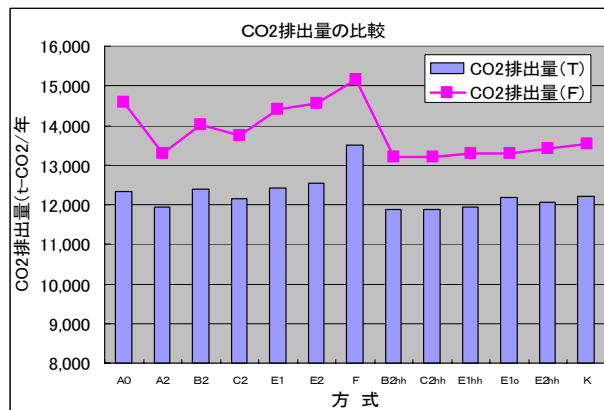
Figure 7 CO 2 Exhaustion
