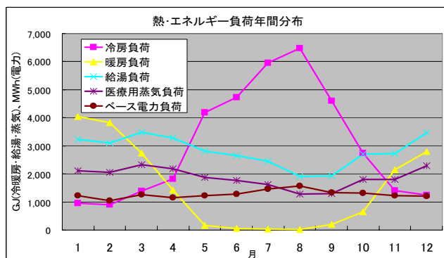
Figure 5 Annual Load
